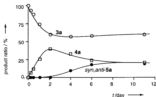
Figure 1. Time-course of the domino reaction of ( \pm )- 3a with 2a .
