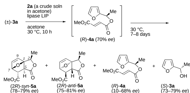
Scheme 4. Lipase LIP-catalyzed domino kinetic resolution/Diels–Alder reaction of ( \pm )- 3a with 2a .
