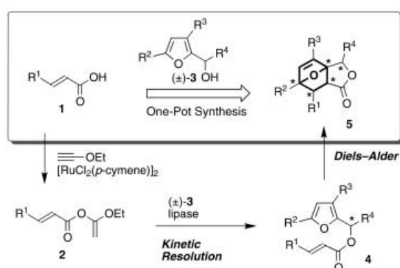
Scheme 2. The domino kinetic resolution/Diels–Alder reaction starting from 1 and (±)- 3 .
