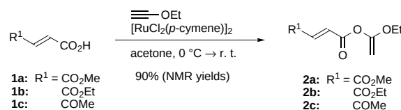
Scheme 3. Preparation of 2a–c from 1a–c .
