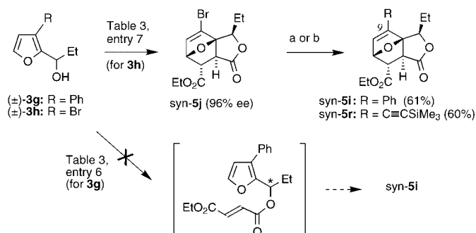
Scheme 6. Preparation of syn - 5i and 5r having a bulky substituent. a) PhB(OH) 2 , PdCl 2 (PPh 3 ) 2 , Na 2 CO 3 , THF, 65 °C; b) (trimethylsilyl)acetylene, Pd(PPh 3 ) 4 , CuI, Et 3 NH, DMF, 50 °C.
