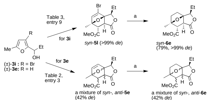
Scheme 5. Preparation of syn - 6e . a) Pd/C, H 2 , MeOH, room temperature.
