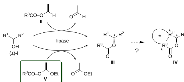
Scheme 1. Transesterification of ( \pm )- I with II or V .
